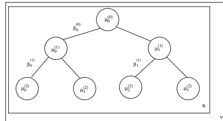
Figure 3: Binary tree representation of multiscale parameters for the case S=2
