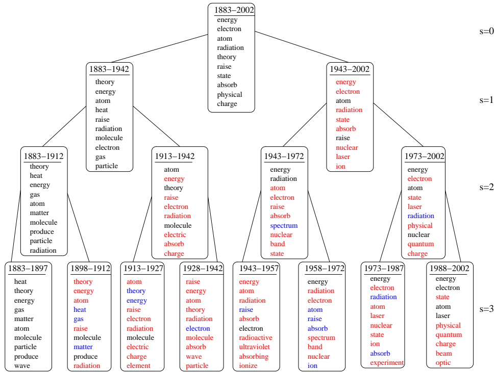
Figure 5: A 4-scale representation of the topic “Particle physics”: words colored red are those whose relative importance in the topic has gone up compared to previous epoch at the same scale. Words colored blue are those whose relative importance has gone down. Words not colored have retained their position compared to previous epoch.
