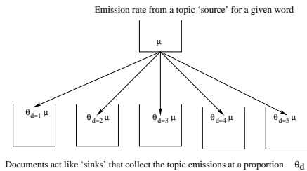
Figure 1: The intuitive idea of Topic Tomography
