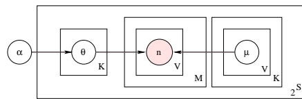
Figure 2: Graphical representation of data generation
