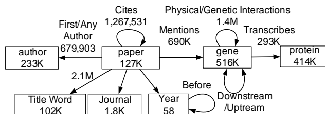
Fig. 2. Schema of the fly data.
