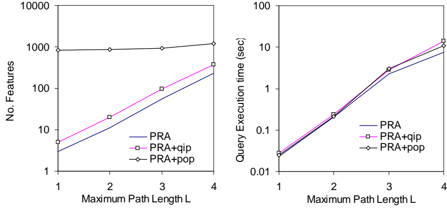
Fig. 4. Model complexity versus maximum path length L for reference recommendation task on the yeast data. Execution time is an average of 2000 test queries.
