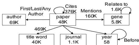
Fig. 1. Schema of the yeast data.
