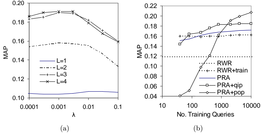
Fig. 5. (a) Compare different regularization parameter \lambda and different path length l . (b) Effect of training data size for reference recommendation task on yeast data
